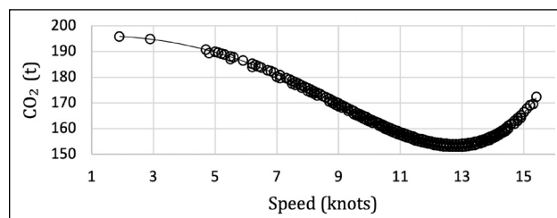
Figure 2. Speed- CO_2 relationship.
