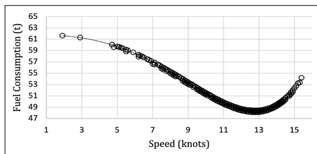
Figure 1. Speed-fuel consumption relationship.
